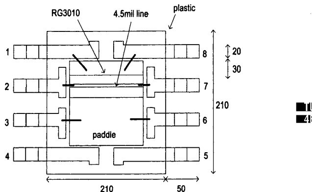
Fig. 1. Classic SSOP8 pin package with 50\Omega through inserted between ports 2 and 7.
