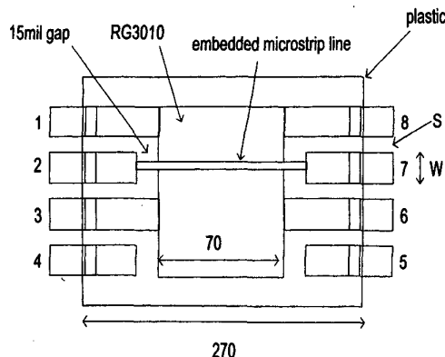
Fig. 5. Proposed modified SSOP8 pin with embedded 50\Omega thru line. The lead pitch is varied to present a 50\Omega characteristic impedance to the bond wire transition. All dimensions in mils.
