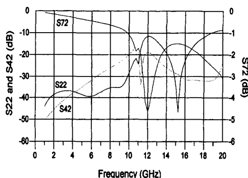
Fig. 6. Fig. 6: HFSS simulation of proposed modified SSOP8 ECPWFG package, showing improved performance to 10 GHz. The lower frequency resonances have been minimized by redesign of the lead frame transitions.
